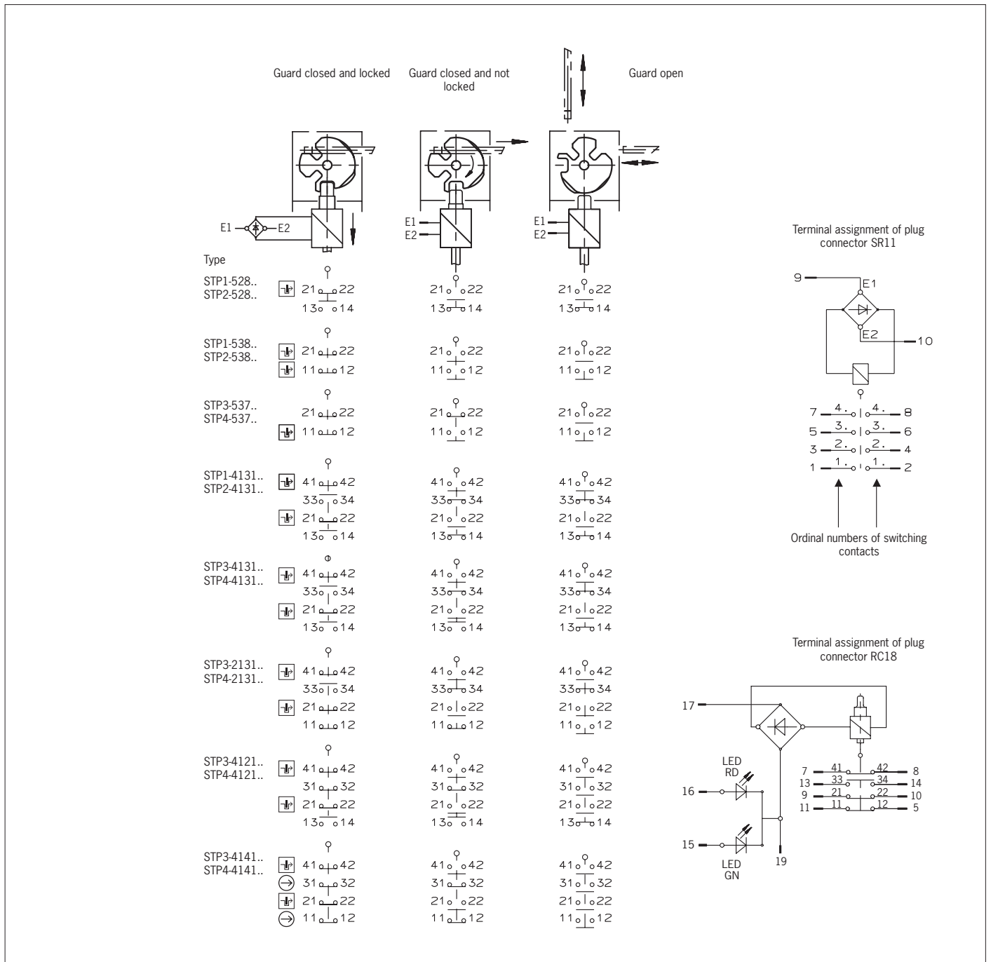
Fig. 3: Switching elements and switching functions
