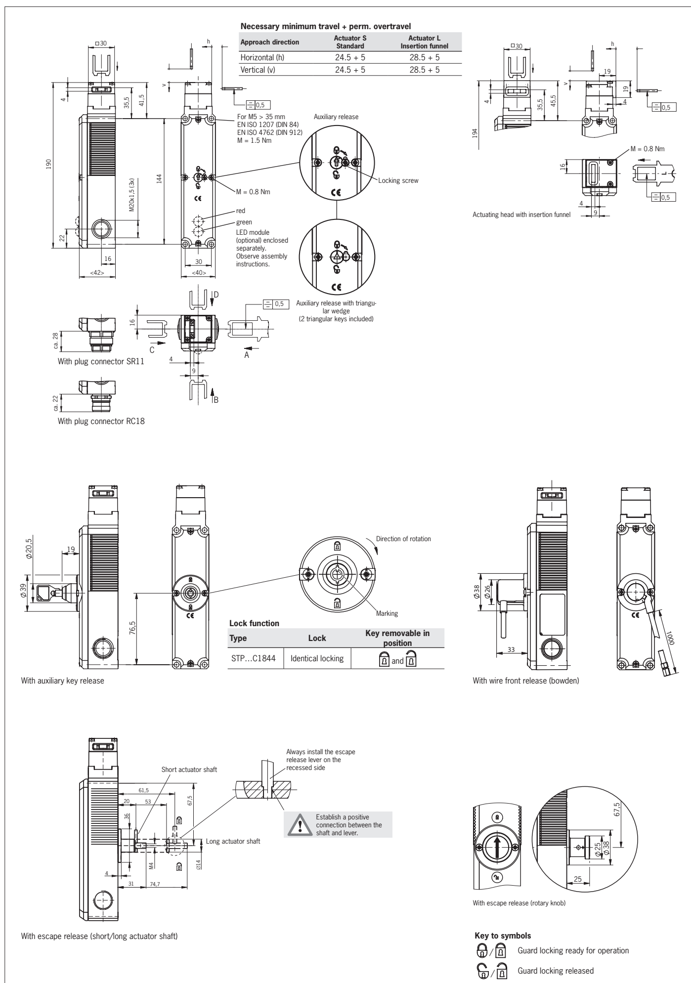
Fig. 2: Dimension drawing for STP... without insertion funnel and STP... with insertion funnel
